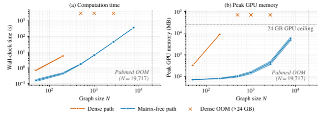
Figure 7: Dense vs. matrix-free AEGIS pipeline (RTX 4090). Dense scales as O((Nd)^3) , exceeding 24 GB beyond N=200 ; matrix-free is roughly O(N \log N) in time, sub-linear in memory, reaching Amazon Photo ( N=7,650 ) at 365 s/5.5 GB.
