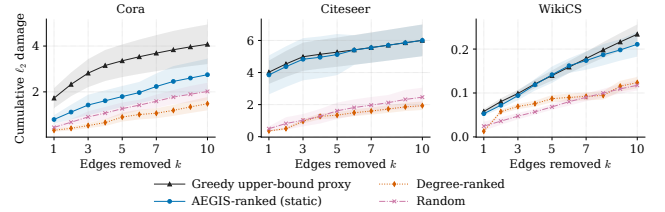
Figure 5: Cumulative damage from sequential discrete edge removal vs. k (IGNN, 50-node subgraph, 10 seeds, \pm 1 sd). AEGIS matches the ground-truth-aware Greedy attacker on Citeseer/WikiCS and recovers 54–67% of Greedy’s damage on Cora at k=5 –10 without any access to discrete ground truth ; degree-ranked stays below random on Cora at every k .
