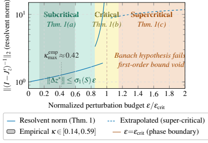
Figure 10: Three-regime characterization of Theorem 1. The empirical \kappa band (grey) saturates well below the spectral-normalization ceiling, so the empirical resolvent growth is far milder than the worst-case 1/(1 - \kappa) divergence at \varepsilon \rightarrow \varepsilon_{\text{crit}} .
