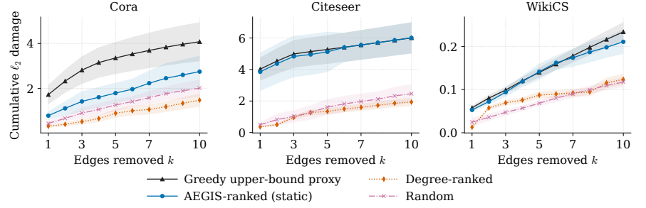
Figure 4: Cumulative damage from sequential discrete edge removal vs. k (IGNN, 50-node subgraph, 10 seeds). AEGIS matches the label-aware Greedy attacker on Citeseer/WikiCS and recovers 54–67% of its Cora damage at k=5-10 with no discrete-label access; degree-ranking stays below random.
