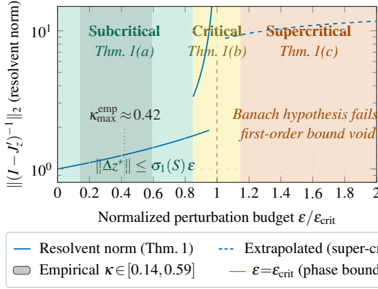
Figure 7: Three-regime characterisation of Theorem 1. The empirical \kappa band (grey) saturates well below the spectral-normalisation ceiling, so the empirical resolvent growth is far milder than the worst-case 1/(1 - \kappa) divergence at \epsilon \rightarrow \epsilon_{crit} .
