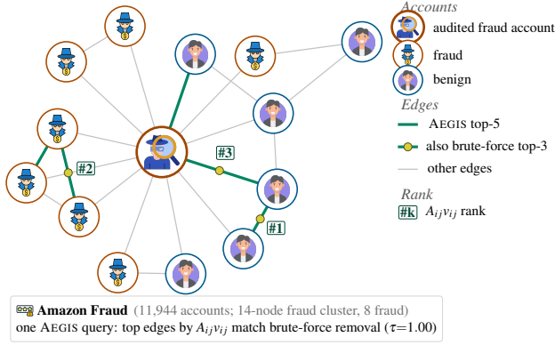
Figure 6: AEGIS auditing an IGNN fraud detector on an Amazon Fraud cluster (Dou et al. 2020). Icons mark fraud / benign accounts; the audited account sits at the hub. Green edges are the top-5 adversarial fault lines by the edge-weighted score A_{ij}v_{ij} ; yellow dots mark the three also in the brute-force single-edge-removal damage top-3.
