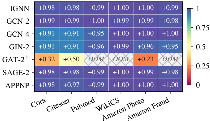
Kendall \tau : continuous \rightarrow discrete transfer
