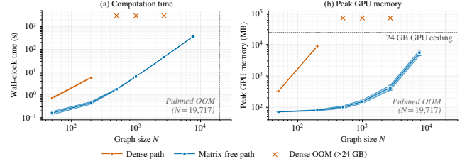
Figure 8: Dense vs. matrix-free AEGIS pipeline (RTX 4090). Dense scales as O((Nd)^3) , exceeding 24 GB beyond N=200 ; matrix-free is roughly O(N \log N) in time, sub-linear in memory, reaching Amazon Photo ( N=7,650 ) at 365 s/5.5 GB.
