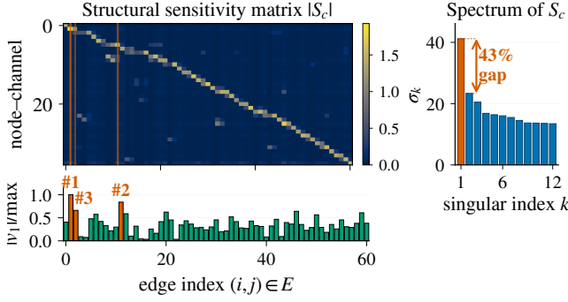
Figure 2: |S_c| on a 50-node Cora ego-graph (IGNN, N=50 , d=16 , |E|=61 , seed 0). Vermilion lines: top-3 edges by |v_1| (SVD-optimal direction, bar strip). Sidebar: singular spectrum ( \sigma_1=41.2 , 43% gap to \sigma_2 ).
