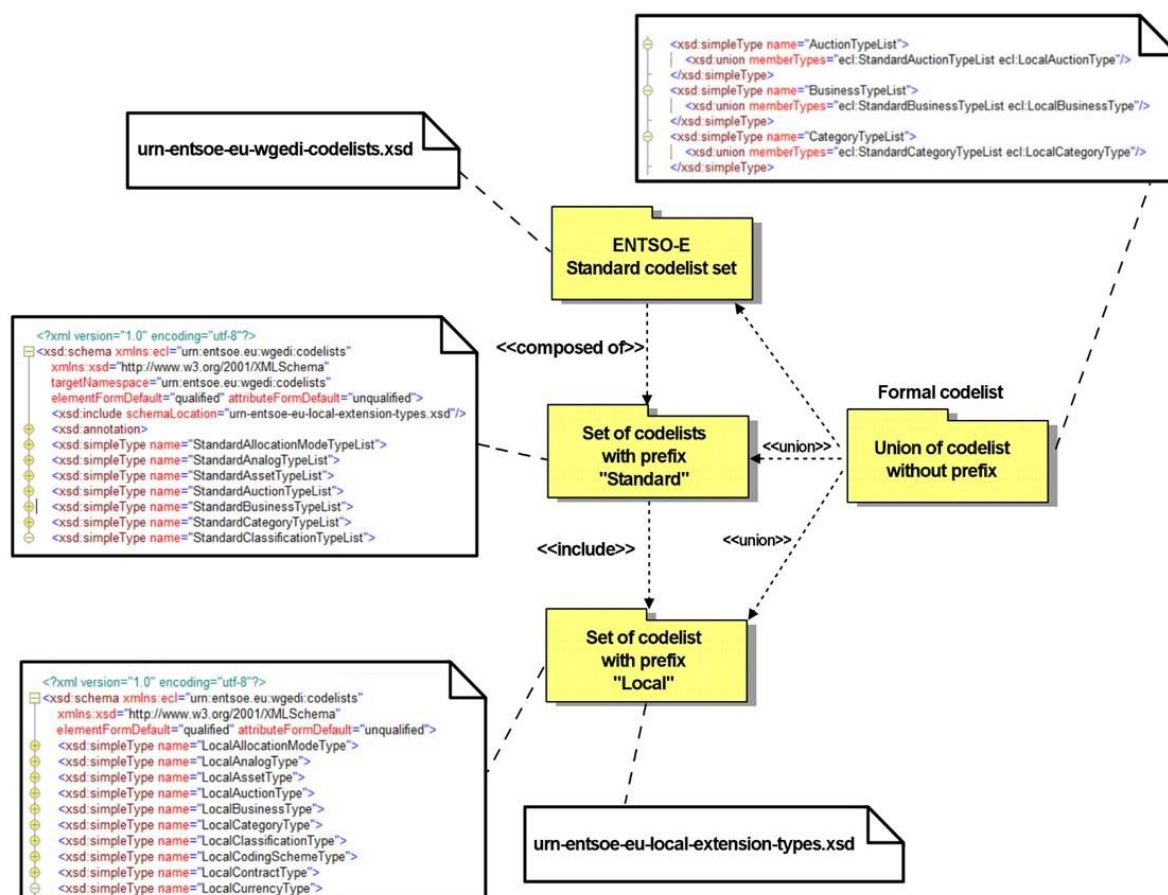
Figure 2 – Codelist schema
