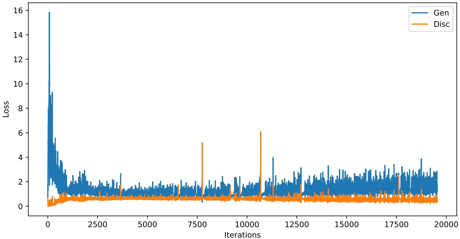
Generator and Discriminator Training Loss
