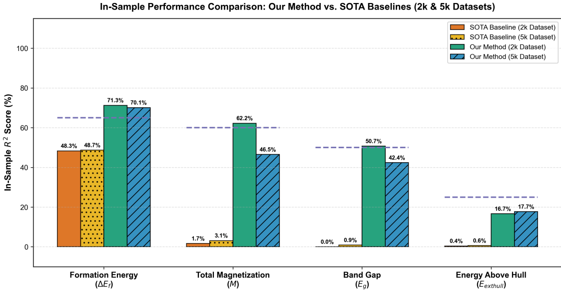
Figure 6: In-sample R^2 score comparison across all four target properties: Our Method vs. literature SOTA baselines (Ouyang 2018, 9 Ghiringhelli 2015, 8 Borlido 2019, 11 Bartel 2019 10 ) and theoretical literature limits ( R^2_{\text{limit}} ).
