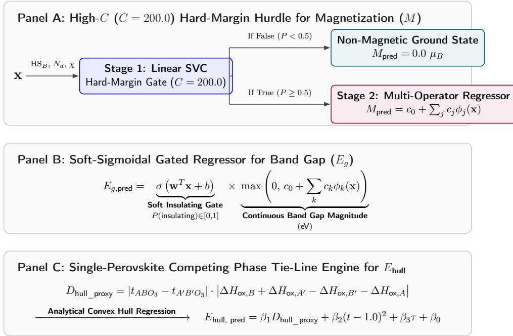
Figure 6: Detailed architectural schematics of the three specialized property-routing mechanisms: (A) High- C Hard-Margin Hurdle Model for magnetization, (B) Soft-Sigmoidal Gated Regressor for band gap, and (C) Single-Perovskite Tie-Line Convex Hull Engine for energy above hull.
