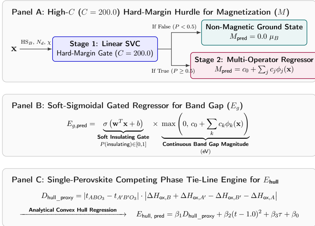
Figure 6: Detailed architectural schematics of the three specialized property-routing mechanisms: (A) High- C Hard-Margin Hurdle Model for magnetization, (B) Soft-Sigmoidal Gated Regressor for band gap, and (C) Single-Perovskite Tie-Line Convex Hull Engine for energy above hull.
