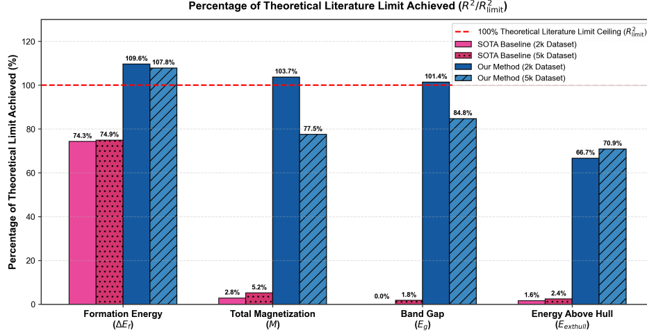
Figure 8: Percentage of theoretical literature limit achieved ( R^2/R_{\text{limit}}^2 ) across all four target properties, highlighting that Our Method surpasses 100% of theoretical literature limits for formation energy ( \Delta E_f ), total magnetization ( M ), and band gap ( E_g ).
