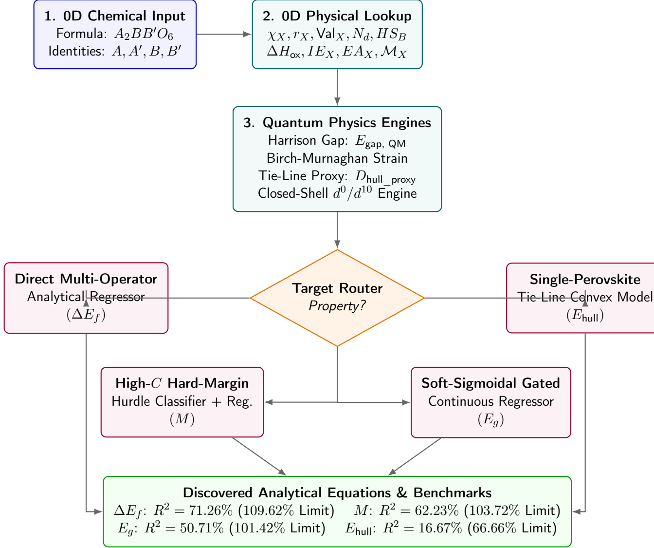
Figure 5: Overall algorithmic architecture of the Master Physics-Gated Double Perovskite Machine Learning Pipeline, showing 0D input ingestion, physics engine expansion, property-specific routing, and final analytical equation outputs.
