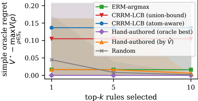
Oracle regret at top- k (HotpotQA, n_{\text{train}} = 400 )
