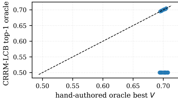
CRRM vs hand-oracle ( k=1 ) win rate 0%, mean \Delta V -0.137
