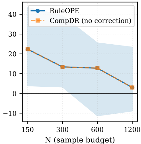
HotpotQA
