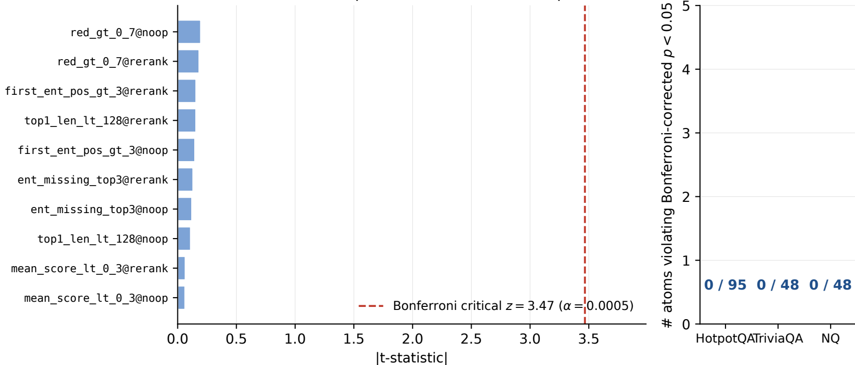
A3 atom-level residual independence (worst 10, HotpotQA × Mistral) Across 3 benchmarks
