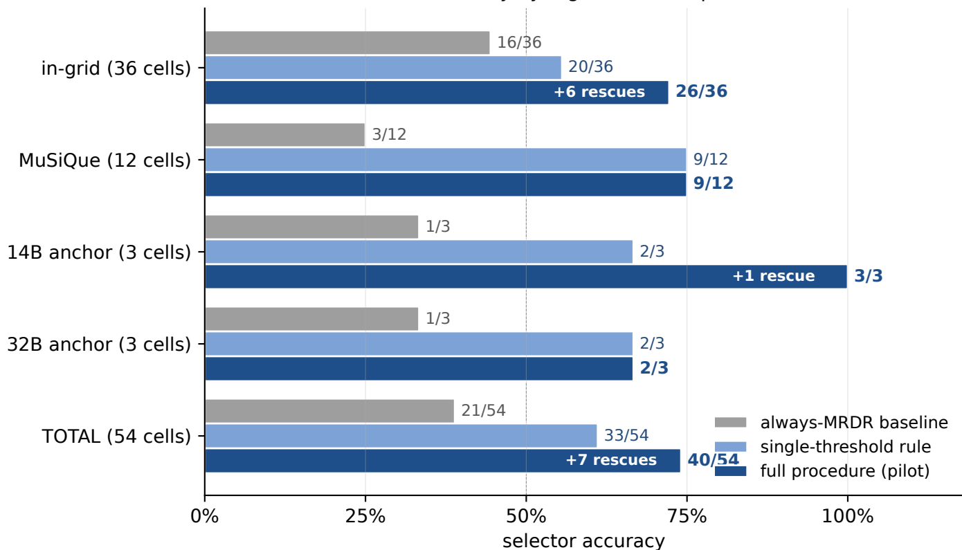
Selector accuracy by regime (54-cell pooled audit)
