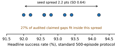
Figure 2: Ten runs of the standard 500-episode LIBERO-10 protocol differing only in flow-sampling seed (5,000 fresh episodes). The 2.2-point spread contains 27% of the 86 recomputable improvements highlighted across the 50 audited papers.
