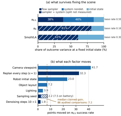
Figure 1: (a) What survives fixing the scene, on the informative task across three policies (base rates 0.16 to 0.59). The replicate block splits that share into flow sampling and system nondeterminism on \pi_{0.5} ; the other two have no replicate block, so only their combined share is measured (hatched). (b) What each factor moves on the reported \pi_{0.5} rate: inference dials the evaluator sets (dark) and deployment shifts (mid). The seed moves the 500-episode aggregate by only 2.2 points because averaging suppresses the per-episode variance in (a); that is the budget the protocol must buy. Dashed line: the median claimed improvement across the audited comparisons.
