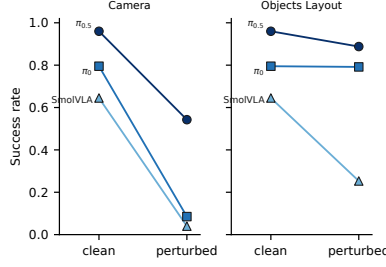
Figure 5: Clean vs. perturbed success for three policies on identical LIBERO-Plus variant sets. Lines never cross (ordering stable) while separations change drastically.
