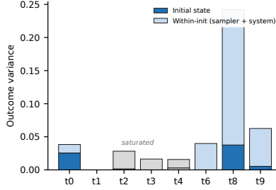
Figure 3: Outcome-variance components per battery task: initial-state share (dark) vs. the within-init component, sampler and system nondeterminism combined (light). On saturated tasks (grey, observed rate \geq 0.96 ) both components collapse: their total outcome variance is at most 0.028, below every non-saturated task.
