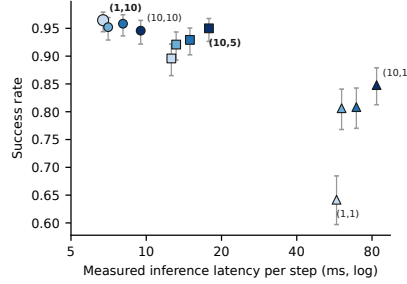
Figure 4: Success rate vs. measured inference latency for all 12 (num\_steps, exec\_horizon) cells ( n=480 each, Clopper–Pearson 95% intervals; latency measured server-side from the episode records). For \pi_{0.5} the published default (10, 5) is dominated; the frontier is a single integration step at horizon 10 (Sec. 6.2 for what replicates on \pi_0 ).
