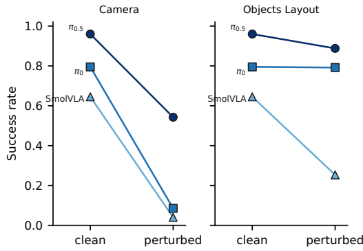
Fig. 5. Clean vs. perturbed success for three policies on identical LIBERO-Plus variant sets. Lines never cross (ordering stable) while separations change drastically.
