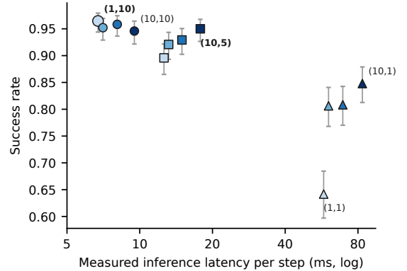
Fig. 1. Success rate vs. measured inference latency for all 12 ( num\_steps, exec\_horizon ) cells ( n=480 each, Clopper–Pearson 95% intervals; latency measured server-side from the episode records). For \pi_{0.5} the published default (10, 5) is dominated; the frontier is a single integration step at horizon 10 (Sec. IV-B for what replicates on \pi_0 ).
