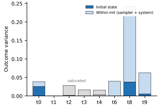
Fig. 4. Outcome-variance components per battery task: initial-state share (dark) vs. the within-init component, sampler and system nondeterminism combined (light). On saturated tasks (grey, observed rate \geq 0.96 ) both components collapse: their total outcome variance is at most 0.028, below every non-saturated task.
