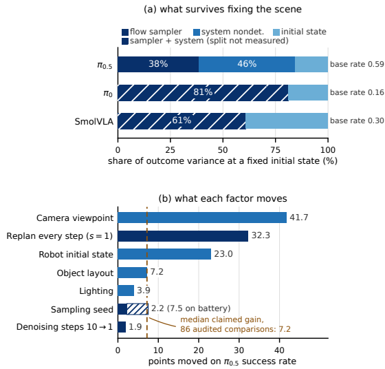
Fig. 2. (a) What survives fixing the scene, on the informative task across three policies (base rates 0.16 to 0.59). The replicate block splits that share into flow sampling and system nondeterminism on \pi_{0.5} ; the other two have no replicate block, so only their combined share is measured (hatched). (b) What each factor moves on the reported \pi_{0.5} rate: inference dials the evaluator sets (dark) and deployment shifts (mid). The seed moves the 500-episode aggregate by only 2.2 points because averaging suppresses the per-episode variance in (a); that is the budget the protocol must buy. Dashed line: the median claimed improvement across the audited comparisons.
