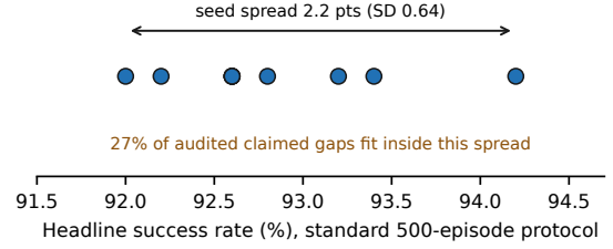
Fig. 3. Ten runs of the standard 500-episode LIBERO-10 protocol differing only in flow-sampling seed (5,000 fresh episodes). The 2.2-point spread contains 27% of the 86 recomputable improvements highlighted across the 50 audited papers.
