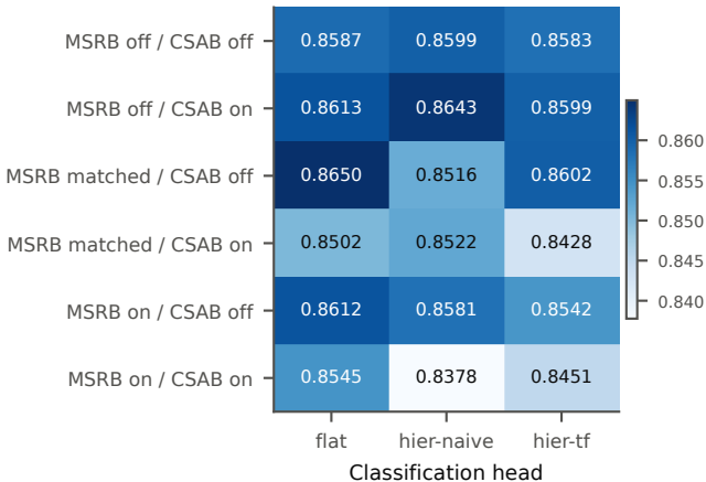
Test macro-F1, 54-run balanced factorial (18 cells \times 3 seeds)
