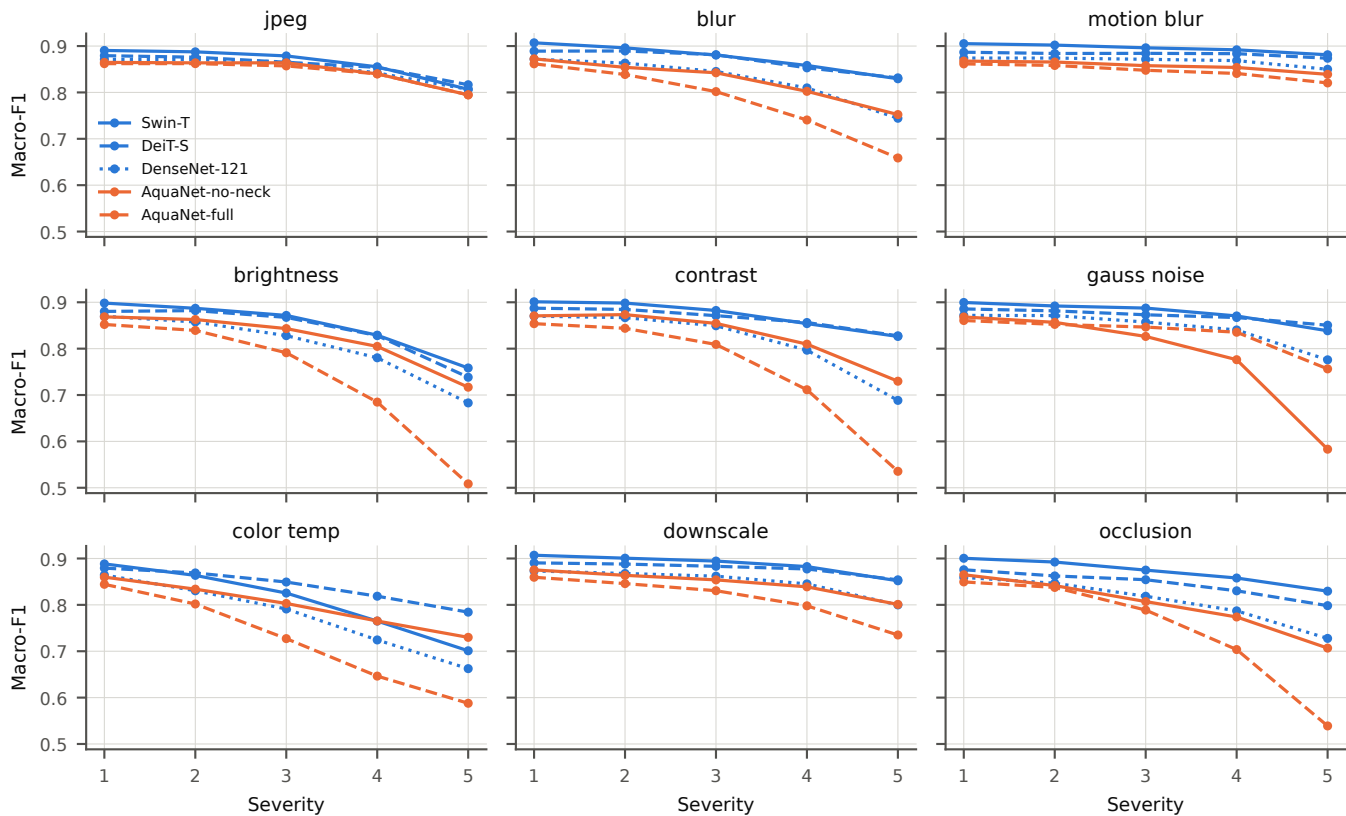
Corruption robustness, mean over five seeds
