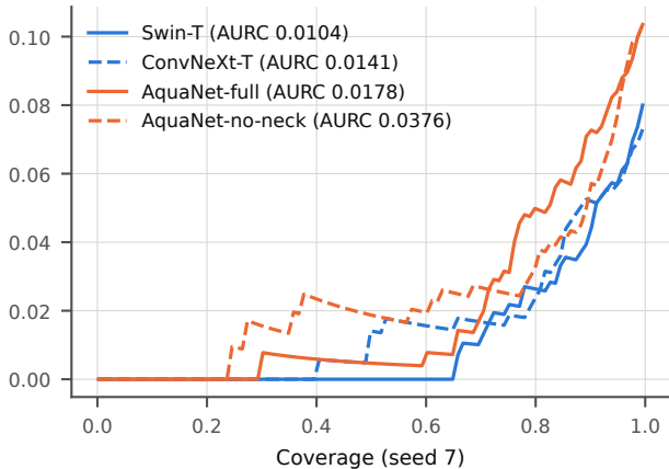
Selective risk
