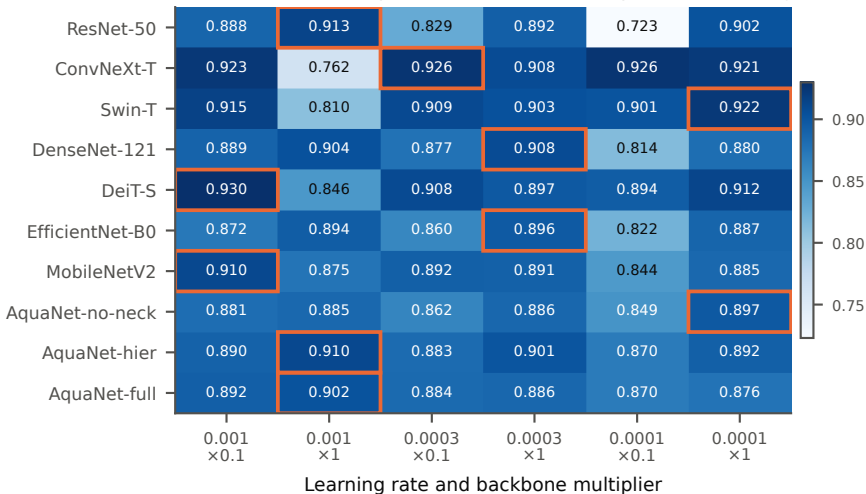
Validation macro-F1 per trial; box marks the promoted setting
