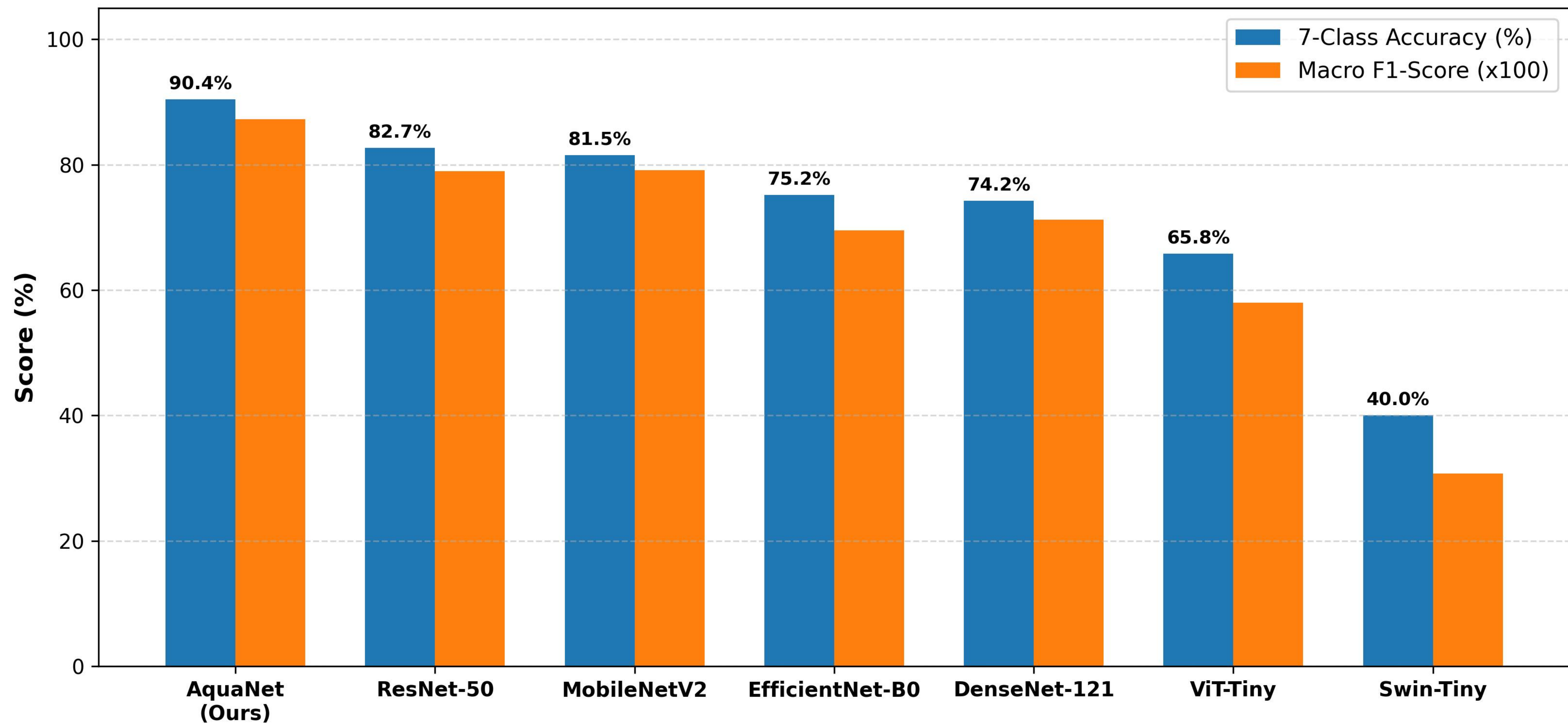
Master Benchmark Model Performance on Un-leaked Test Set
