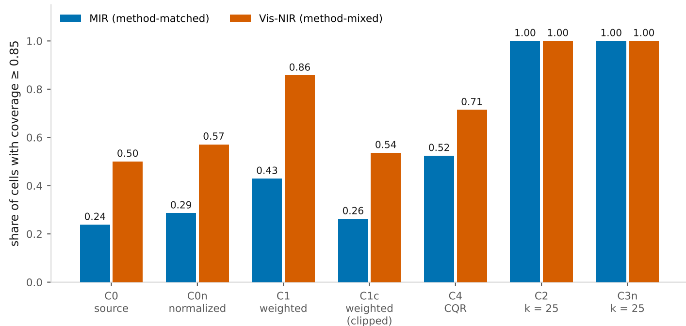
Figure 2. Reliability: in how many libraries the method actually works
