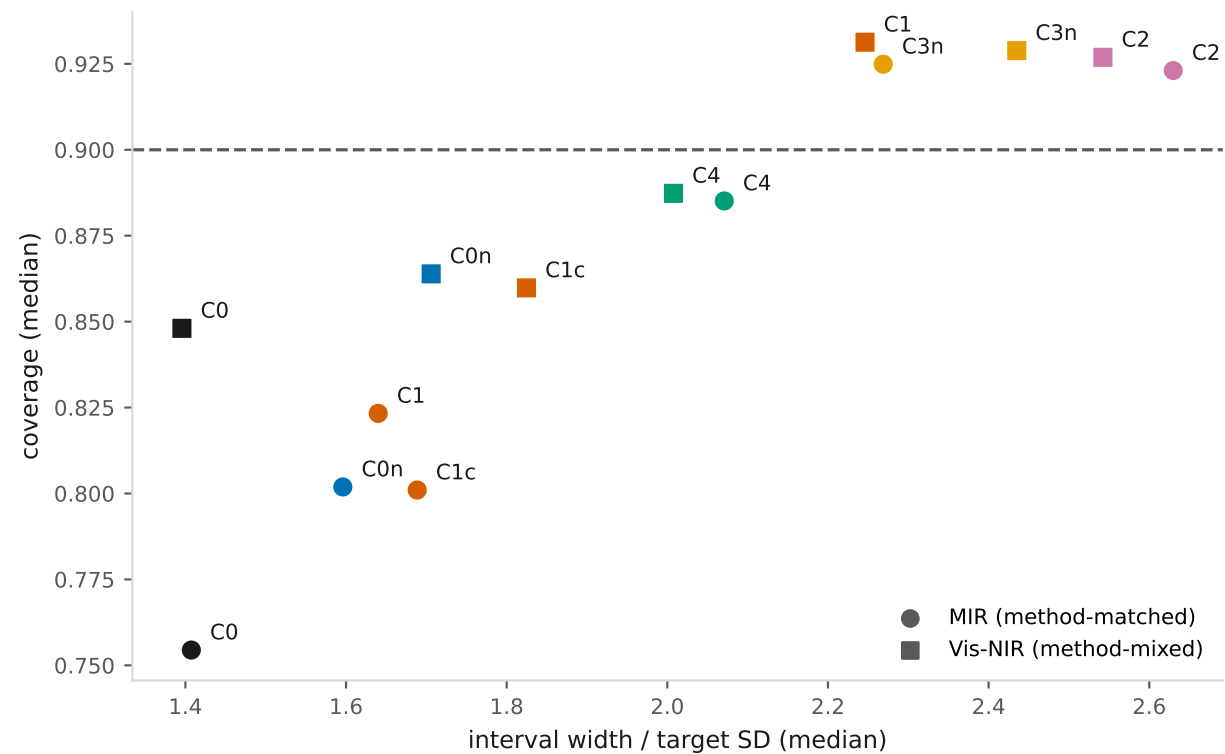
Figure 4. Valid intervals are paid for in width
