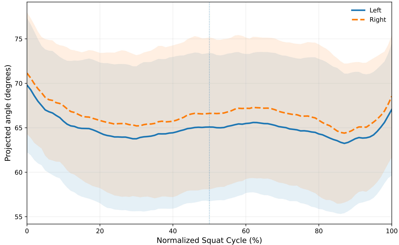
Front View — Ankle Left-Right Trajectory
