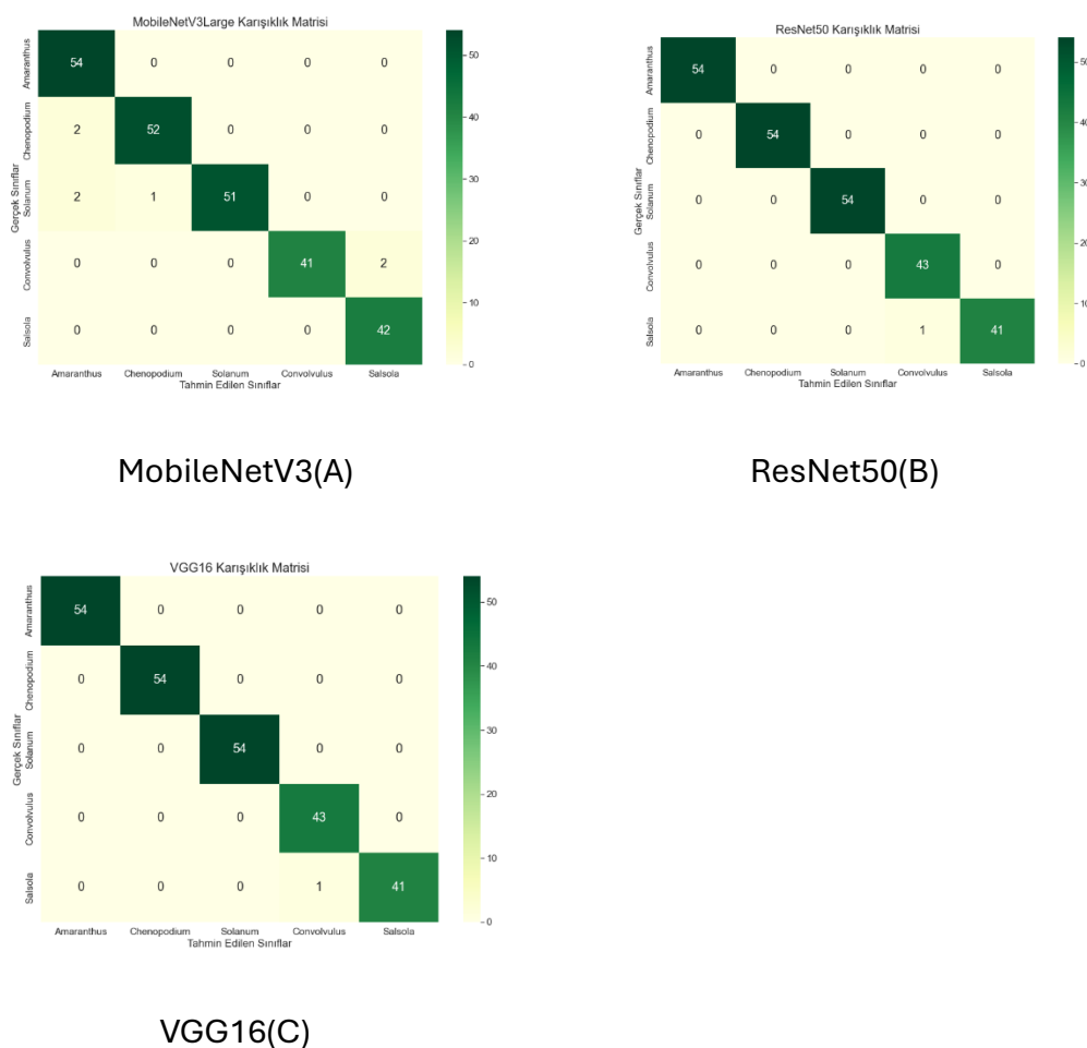
Figure 7: Confusion matrices
