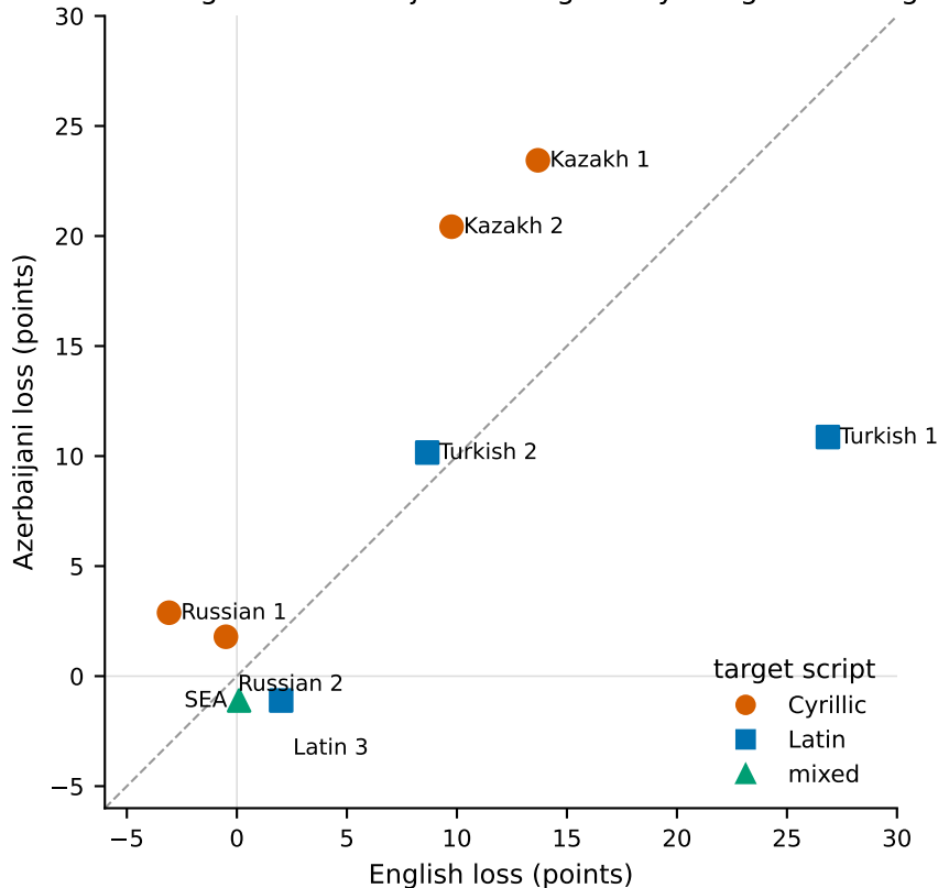
Above the diagonal: Azerbaijani damaged beyond general forgetting
