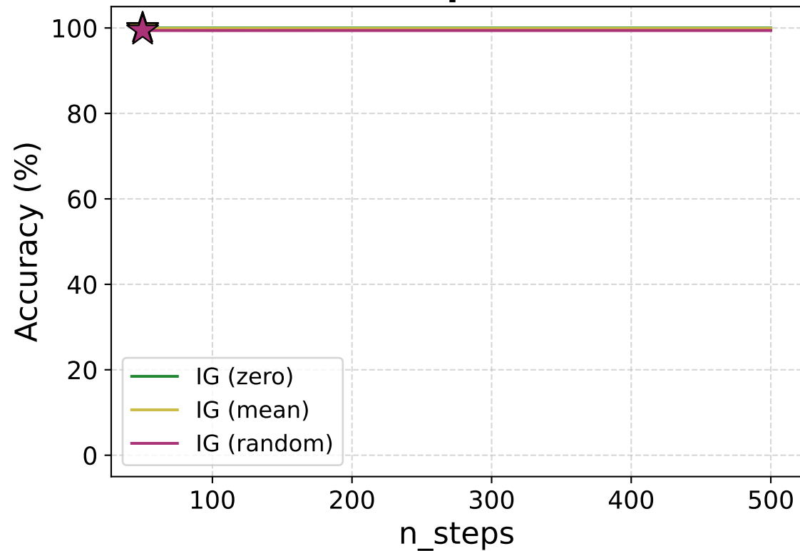
Top-1
