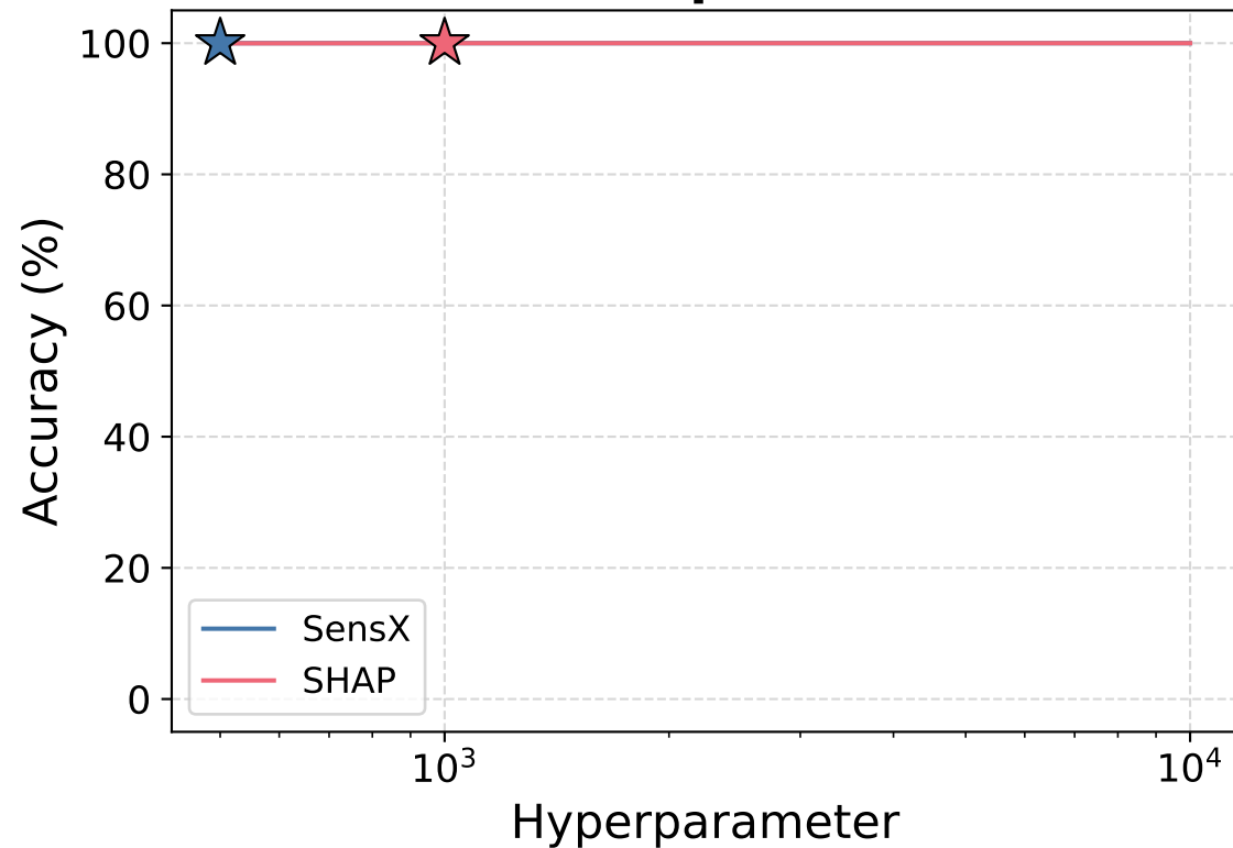
Top-1
