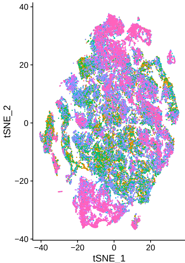
t-SNE by orig.ident
