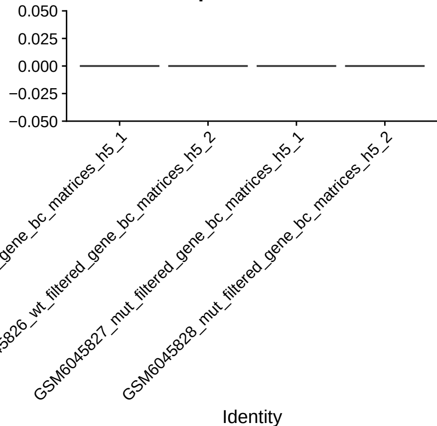
percent.mt
