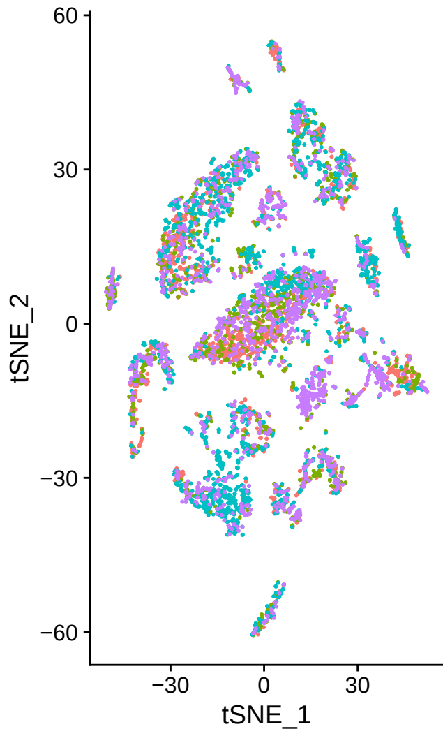
t-SNE by orig.ident
