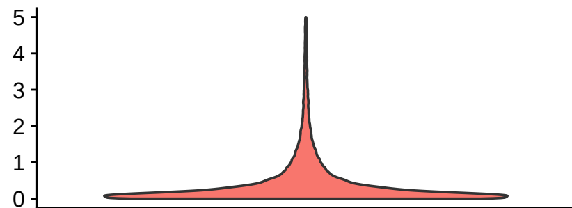
percent.mt
