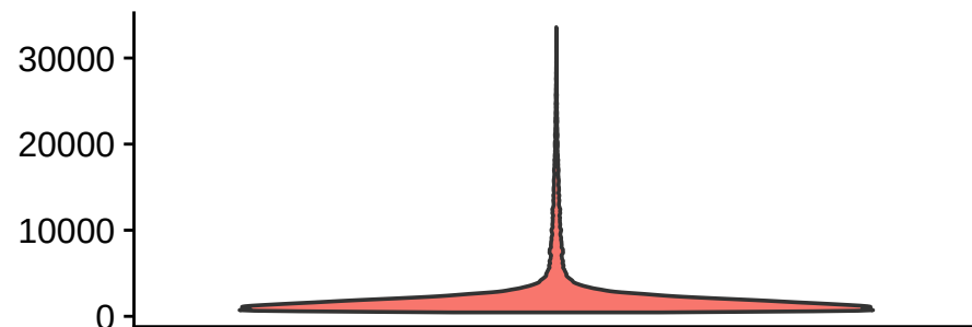
nCount_RNA
