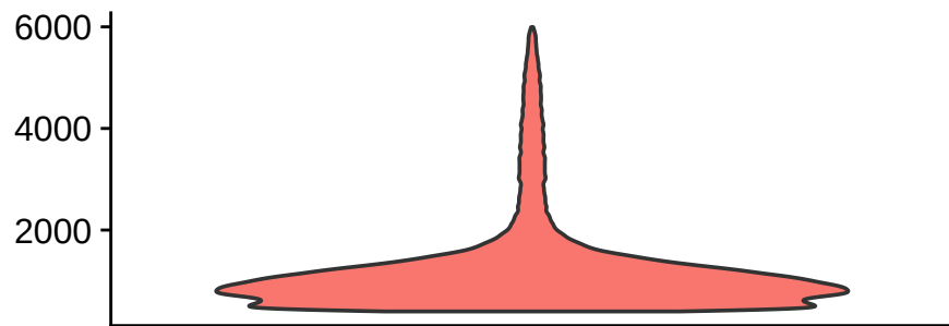
nFeature_RNA
