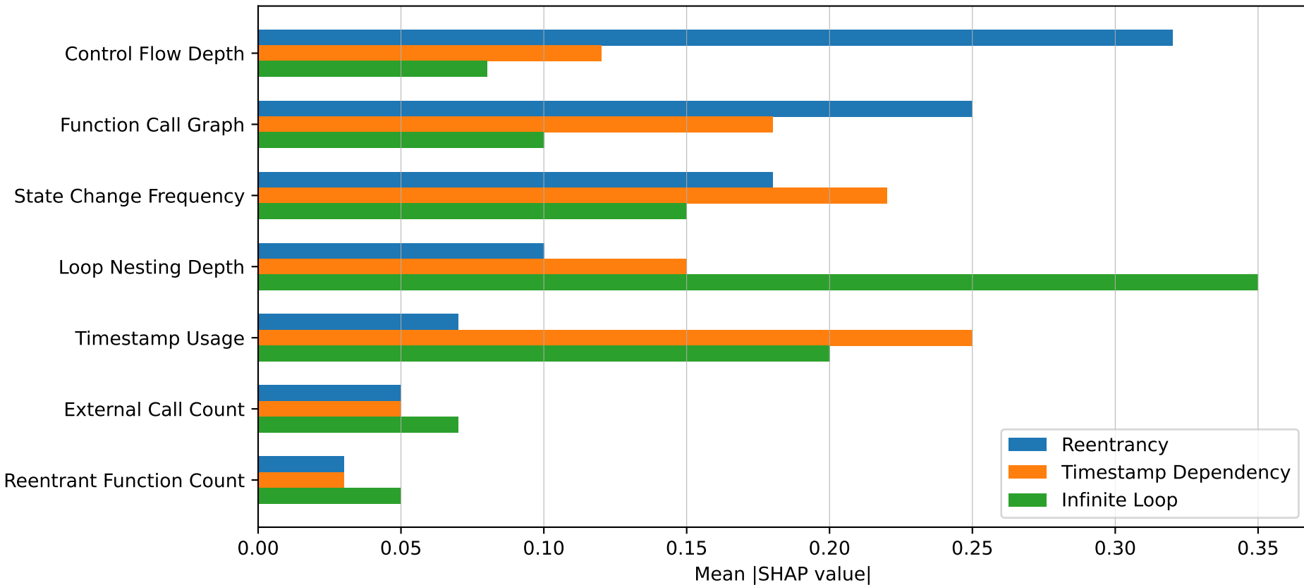
Feature importance (SHAP)
