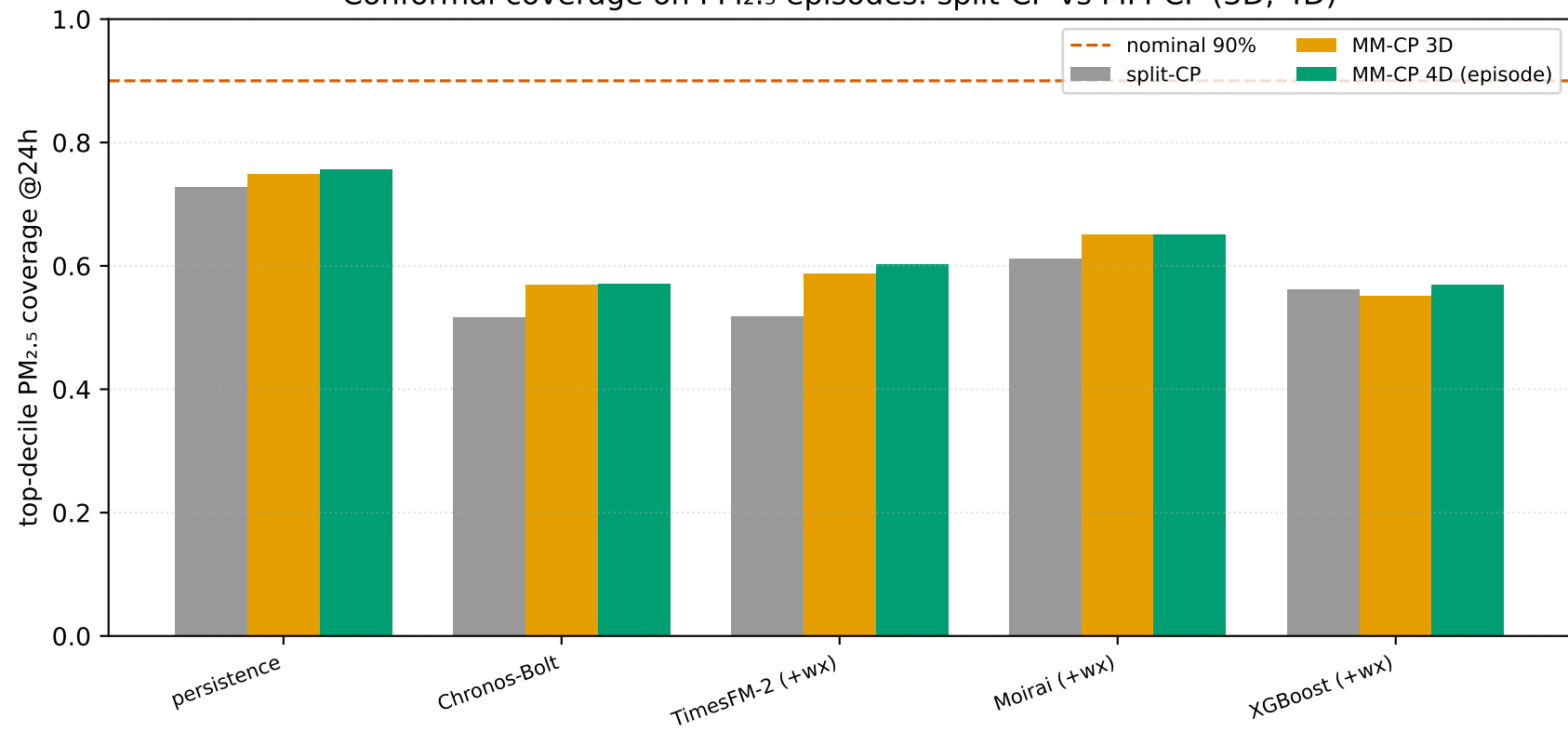
Conformal coverage on PM 2.5 episodes: split-CP vs MM-CP (3D, 4D)
