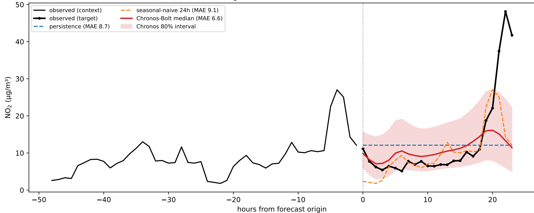
AQ-FM-Bench PoC — Sheffield Devonshire Green NO 2 , 24h forecast origin 2024-06-01 00:00 UTC
