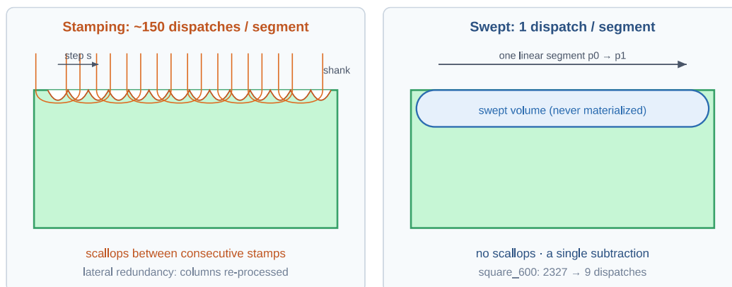
Stamping (baseline) vs Swept subtraction
