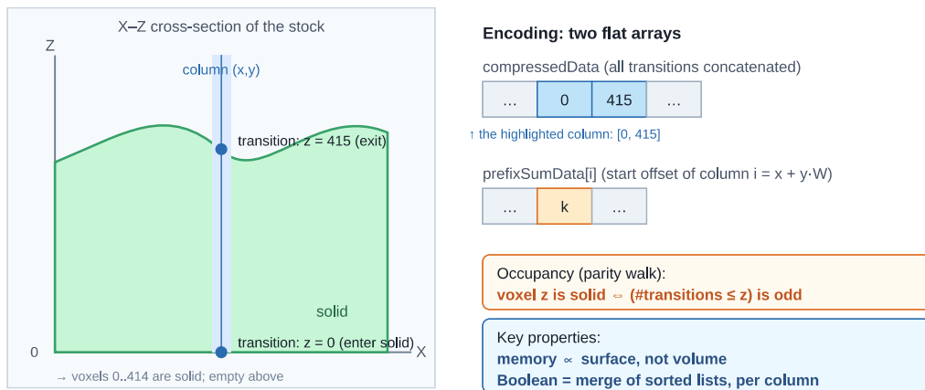
Figure 1. The single-axis dixel (Z-transition column) representation. Each column stores the sorted heights where occupancy flips; two flat arrays encode the whole object, and occupancy is recovered by a parity walk. Storage is proportional to surface complexity, not volume, and any Boolean operation is a merge of sorted lists, independent per column.
