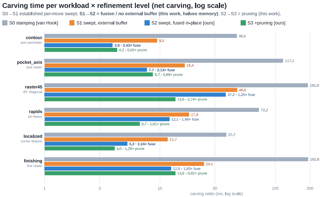
Figure 9. Net carving time per machining workload and refinement level (log scale). S0→S1 is the established per-move swept method; S1→S2 (orange→blue) is this work’s fusion — the swept volume computed on the fly and subtracted in place instead of via a separate buffer (≈1.25–2.4×, and it halves resident memory) ; S2→S3 (blue→green) is this work’s tube-pruning + in-air skip, which pays where the dispatch over-covers (45° raster 2.74×, air-heavy 1.81×).
