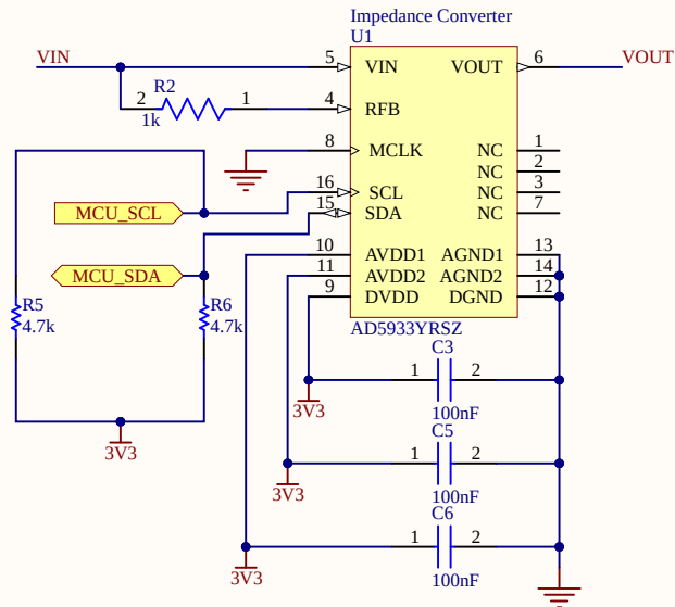
AD5933 Impedance Converter
