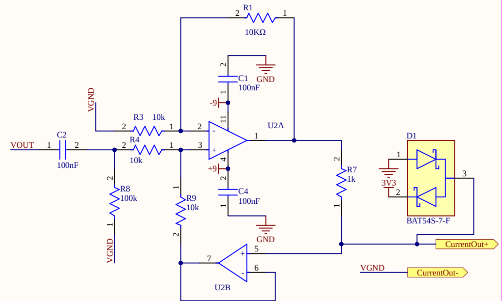
Enhanced Howland Current Pump
