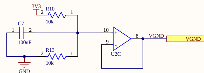
Virtual Ground Generation
