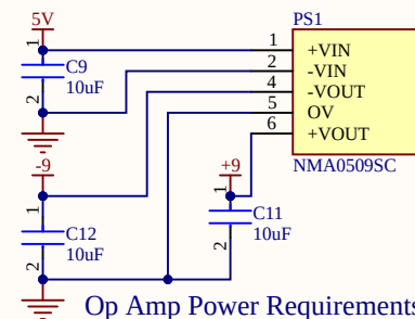
Op Amp Power Requirements
