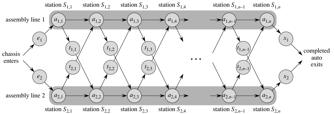
Figure 15.1 A manufacturing problem to find the fastest way through a factory. There are two assembly lines, each with n stations; the j th station on line i is denoted S_{i,j} and the assembly time at that station is a_{i,j} . An automobile chassis enters the factory, and goes onto line i (where i = 1 or 2 ), taking e_i time. After going through the j th station on a line, the chassis goes on to the (j+1) st station on either line. There is no transfer cost if it stays on the same line, but it takes time t_{i,j} to transfer to the other line after station S_{i,j} . After exiting the n th station on a line, it takes x_i time for the completed auto to exit the factory. The problem is to determine which stations to choose from line 1 and which to choose from line 2 in order to minimize the total time through the factory for one auto.
