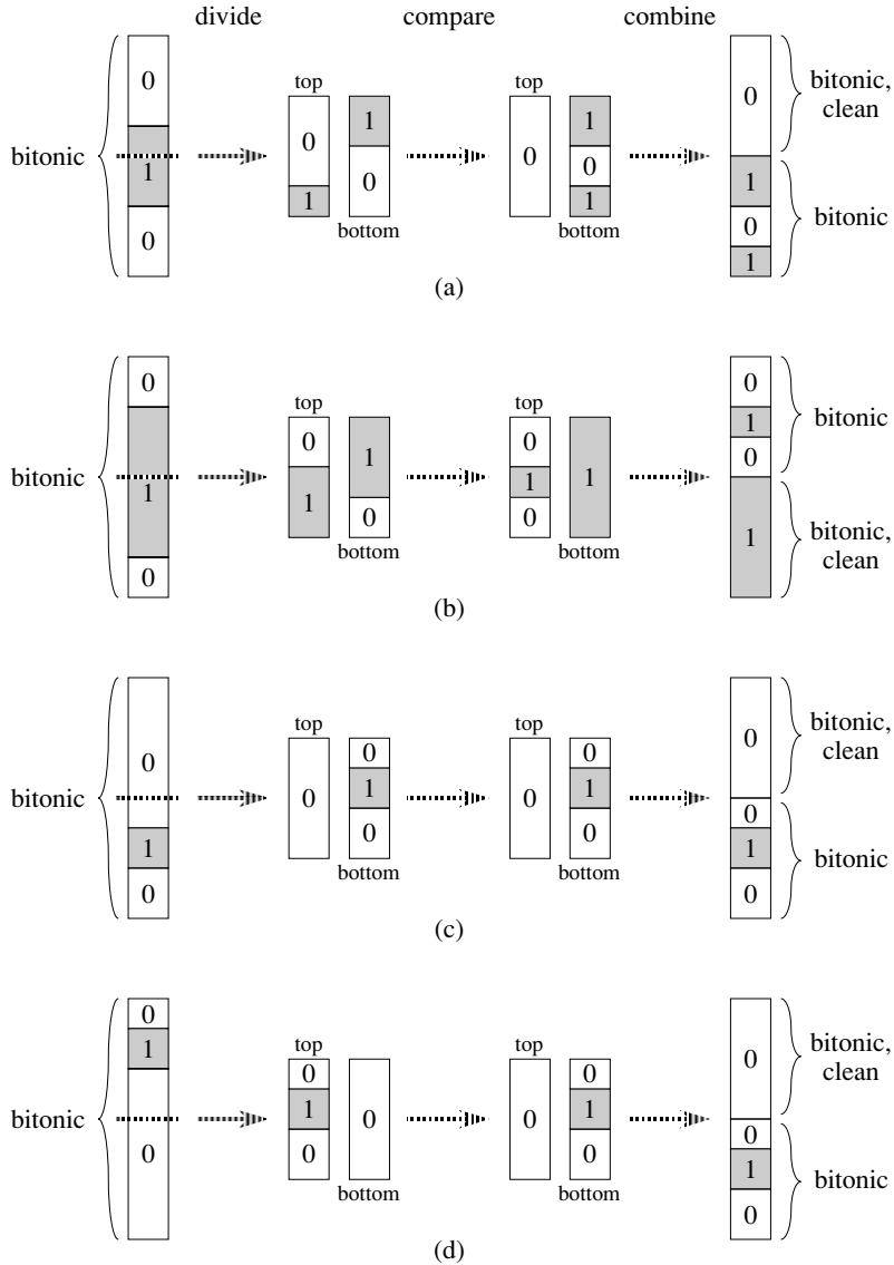
Figure 27.8 The possible comparisons in HALF-CLEANER[n]. The input sequence is assumed to be a bitonic sequence of 0's and 1's, and without loss of generality, we assume that it is of the form 00...011...100...0. Subsequences of 0's are white, and subsequences of 1's are gray. We can think of the n inputs as being divided into two halves such that for i = 1, 2, \dots, n/2 , inputs i and i + n/2 are compared. (a)–(b) Cases in which the division occurs in the middle subsequence of 1's. (c)–(d) Cases in which the division occurs in a subsequence of 0's. For all cases, every element in the top half of the output is at least as small as every element in the bottom half, both halves are bitonic, and at least one half is clean.
