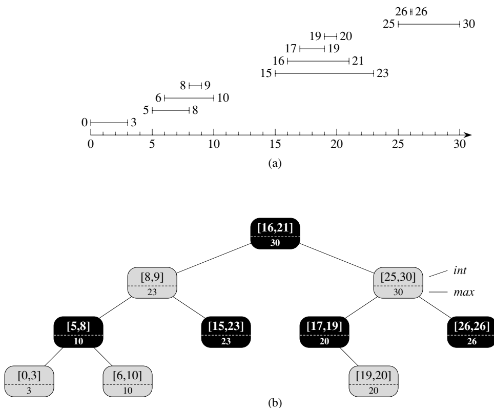
Figure 14.4 An interval tree. (a) A set of 10 intervals, shown sorted bottom to top by left endpoint. (b) The interval tree that represents them. An inorder tree walk of the tree lists the nodes in sorted order by left endpoint.
