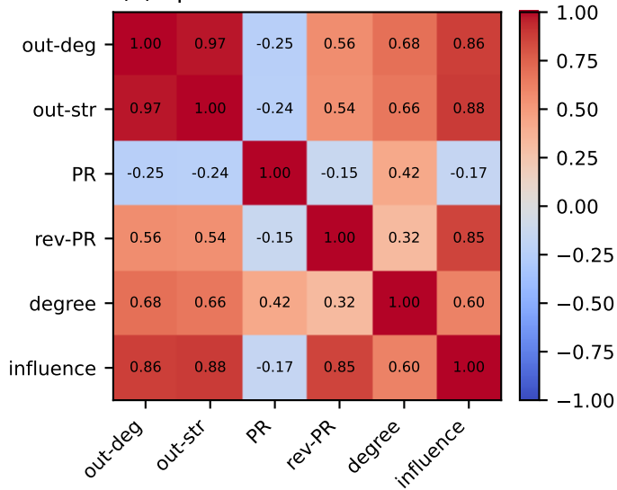
(a) Spearman rank correlations
