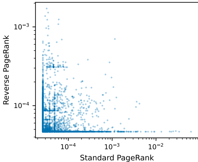
(b) Direction matters (Spearman \rho = -0.15 )
