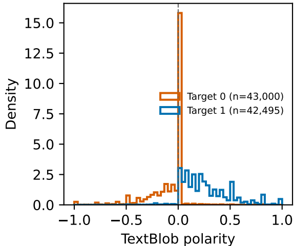
(a) Full-data lexical polarity
