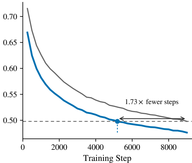
Bengali (out-of-distribution)
