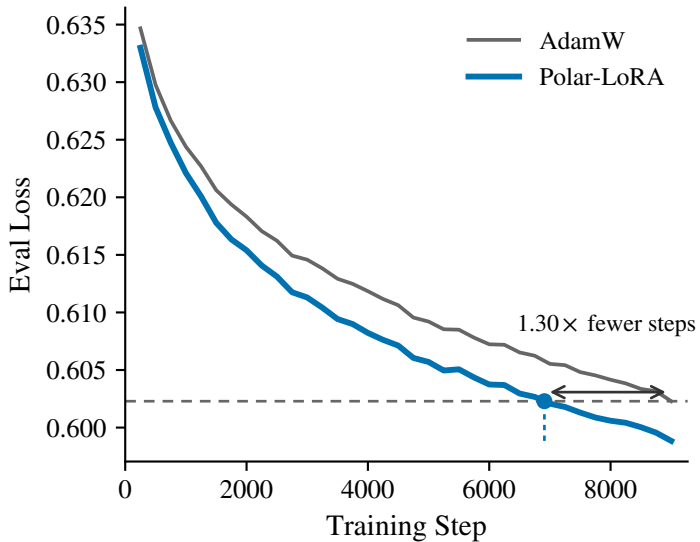
Code (in-distribution)
