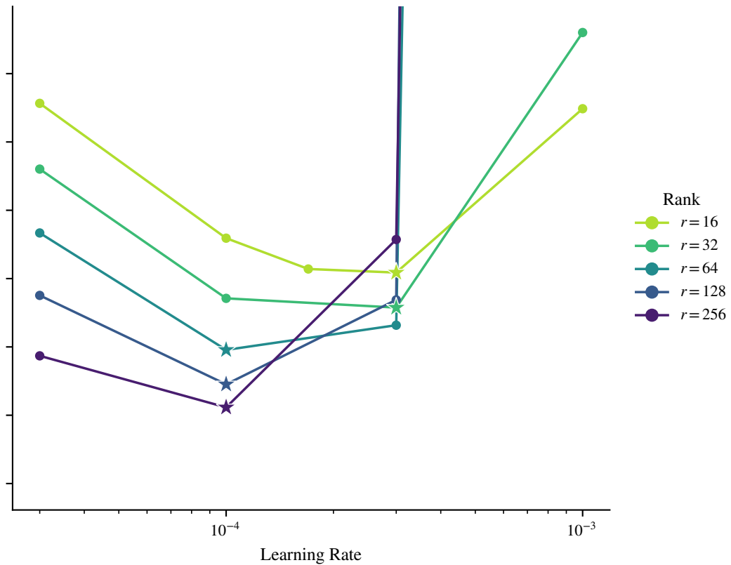
Adam
