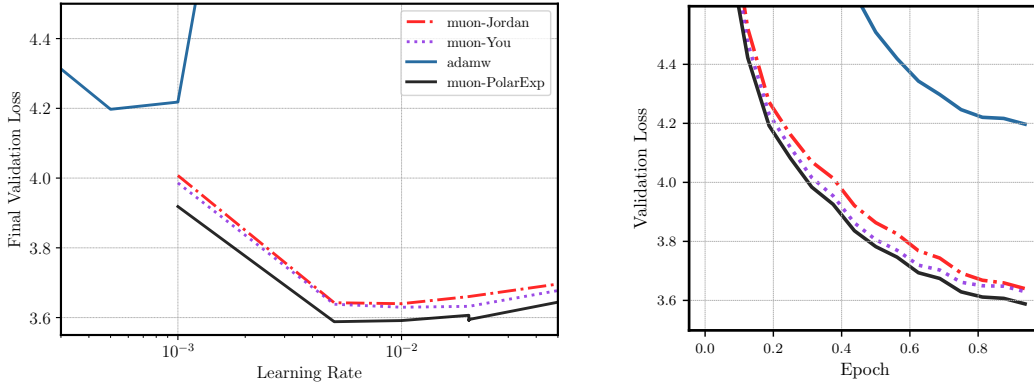
Figure 4: Training a GPT-2-Small (124M) model on 1 Billion tokens of the FineWeb data set (Aroca-Ouellette et al., 2023). muon- <method> denotes Muon with 5 iterations of <method> to compute \text{polar}(M) . No weight decay is used. Left: final validation loss vs. learning rate. The best final validation losses for each method were adamw(lr=0.0005): 4.197, muon-Jordan(lr=0.01): 3.639, muon-You(lr=0.01): 3.629 and muon-PolarExp(lr=0.005): 3.588. Right: Validation loss vs. training iteration.
