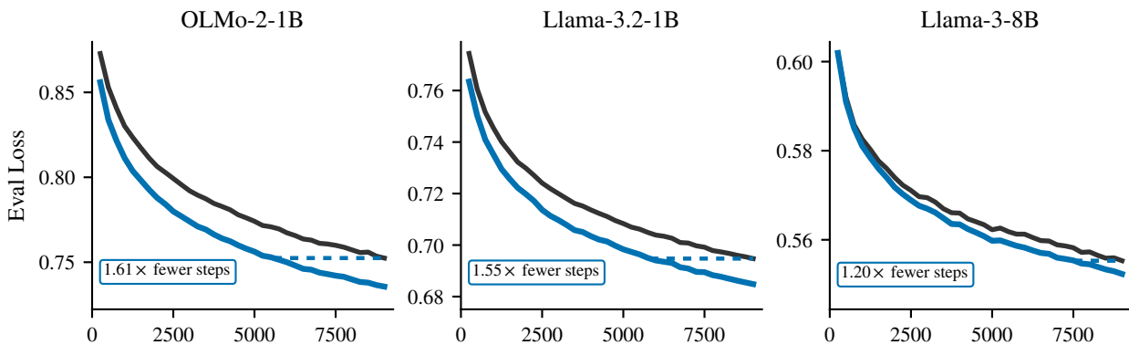
(b) Model families — math ( r=256 )
