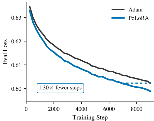
Code (in-distribution)
