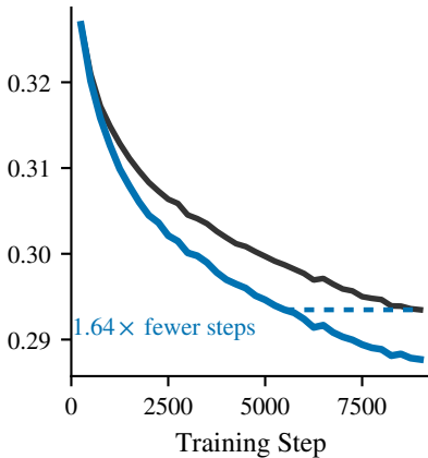
Qwen2.5-1.5B
