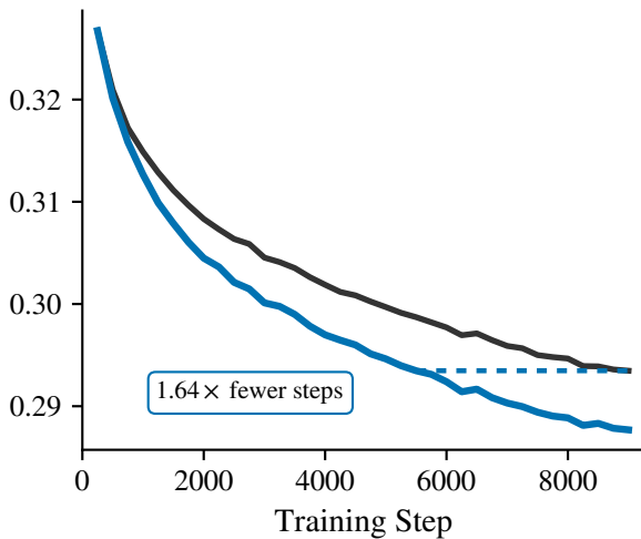
Qwen2.5-1.5B
