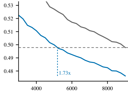
Llama-3.2-1B / OpenMathInstruct-2 / r=64
