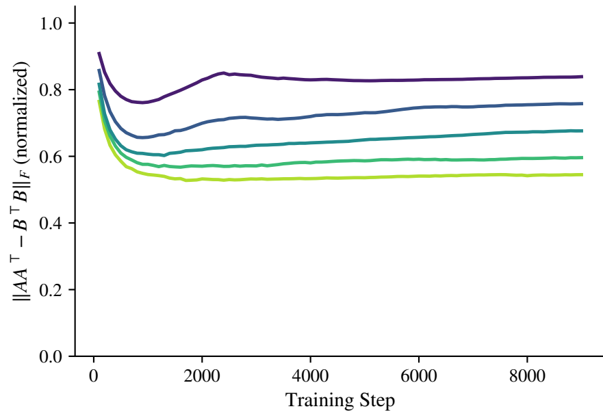
Frobenius Norm Balance
