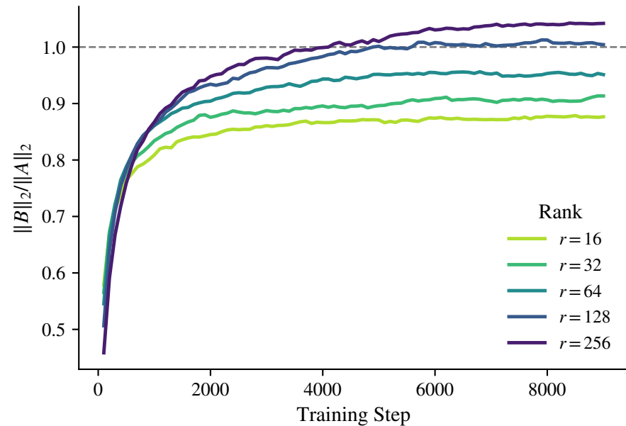
Operator Norm Ratio
